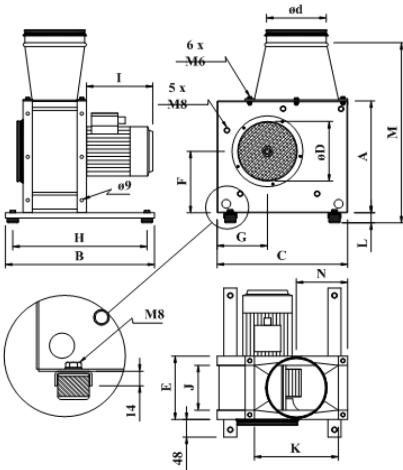
Dimension table Fans LSFG/MSFG 146-250
