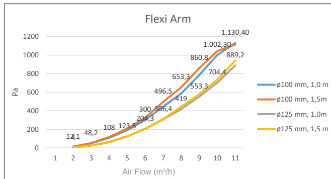
FLEXI arm with Standard ALU hood
