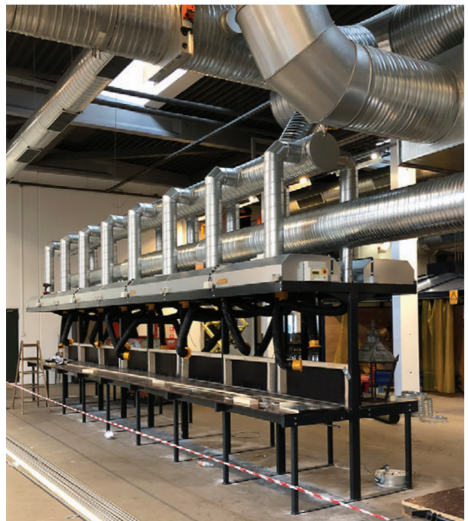
As seen in the picture, the hoods can be mounted in series so that the length of the hood itself can almost become infinite.
