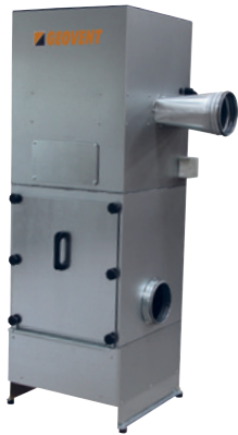
Dustbox with fan and manual compressed air cleaning.
